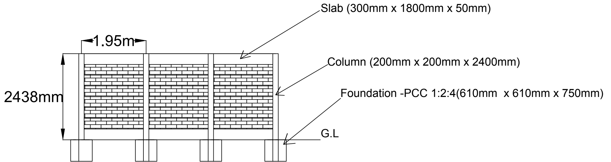
ERECTION DRAWING OF COMPOUND WALL
