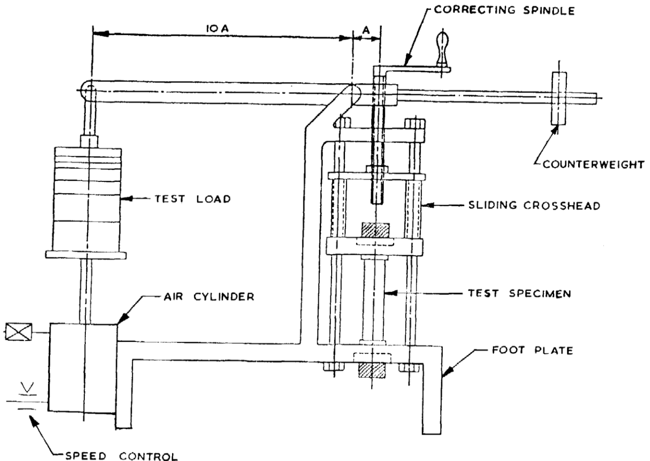
All dimensions in millimetres. Figure --- Diagram of suitable apparatus
