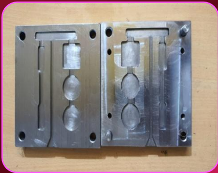
Manufacturing of Die for Specimen Casting
