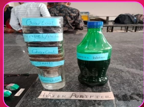
Water purifier using waste plastic bottle
