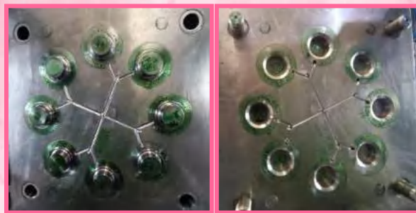
Bulb Holder Cap Mould
