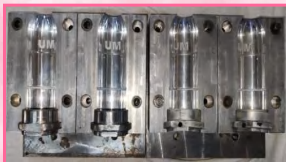
Machining of 200ml PET blow mould
