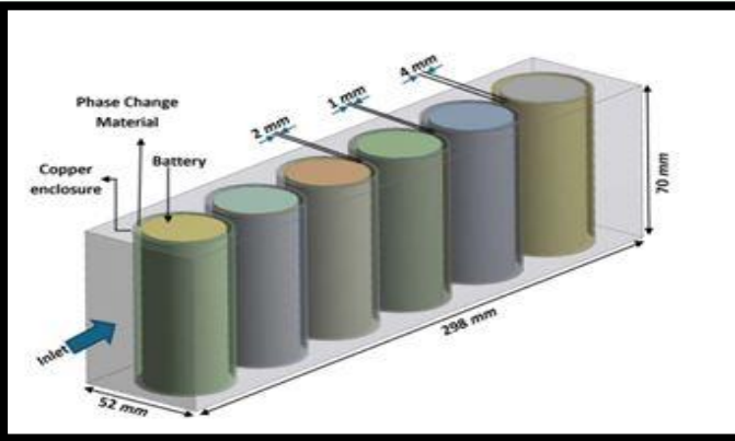
Design & CAD Modelling of Battery Case For Flunt Simulation by Bhopal centre
