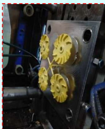
Design & Development of Injection mould for Armature Fan 4 cavity
